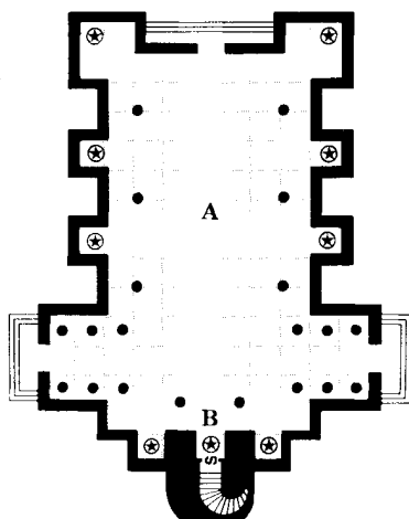
Ground Level
